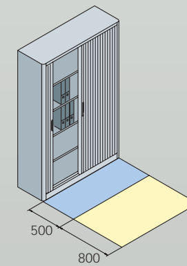
Visualisation of the functional area requirements of a tambour cupboard.
